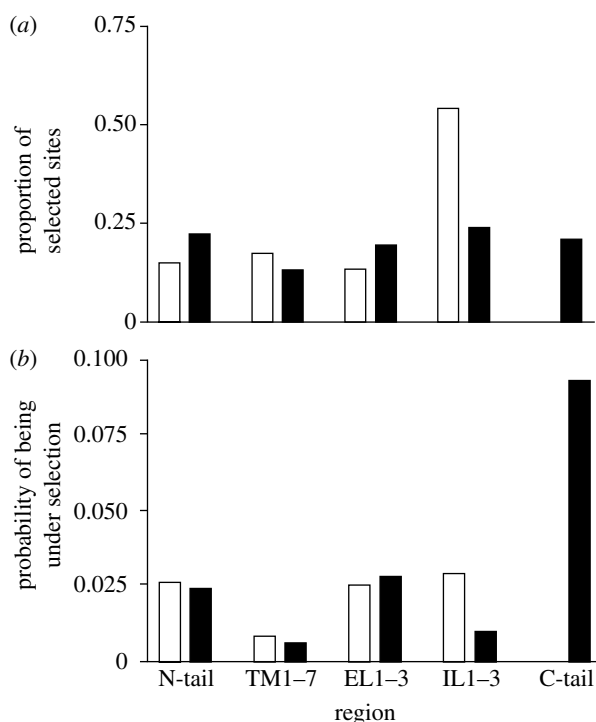
Figure 1. (a) Distribution of the sites showing evidence of divergence by protein regions ( NH_2 -tail, TM domains 1–7 (TM1–7), extracellular loops 1–3 (EL1–3), intracellular loops 1–3 (IL1–3), COOH-tail). (b) The overall probability of an amino acid showing evidence of divergent selection. OR, olfactory receptor (white bars); GR, gustatory receptor (black bars).
